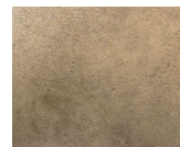
PYRITE
